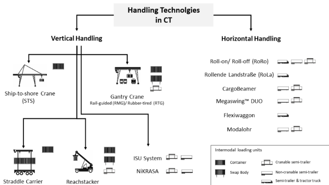
Figure 18: Handling Technologies in Combined Transport
